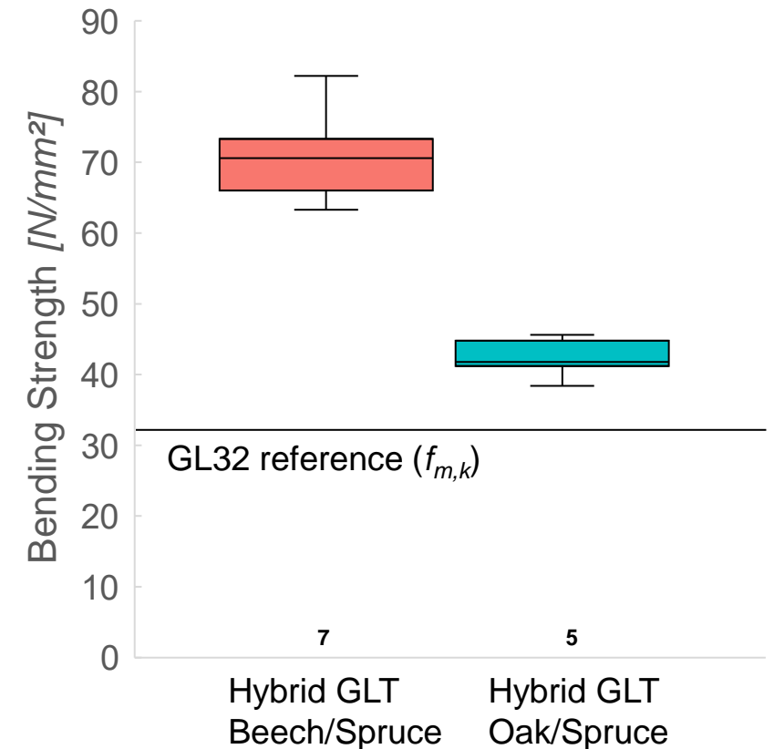
Results of the 4-Point bending tests with references
